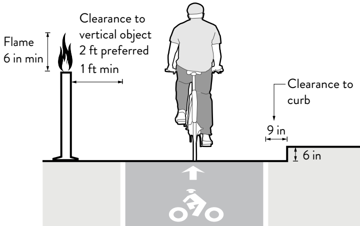
EXHIBIT 5-33: Flaming Separated Bike Lane Elements
